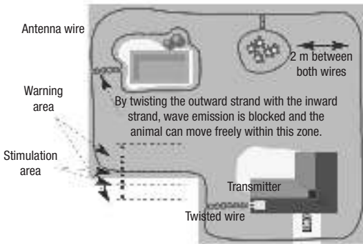
Diagram 3 – Sample installation
